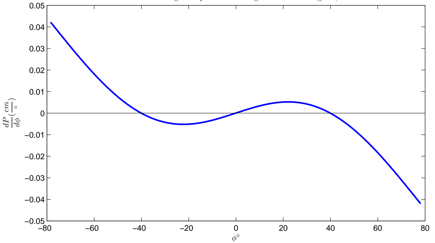
Rate of Change in Optical Path Length "P" Versus angle " \phi "
