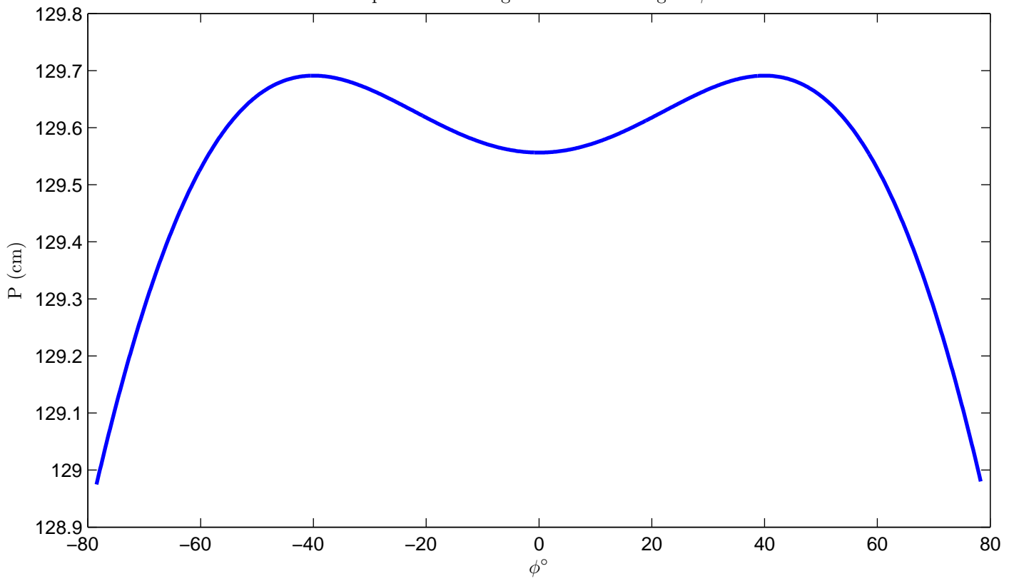
Optical Path Length "P" Versus Angle " \phi "
